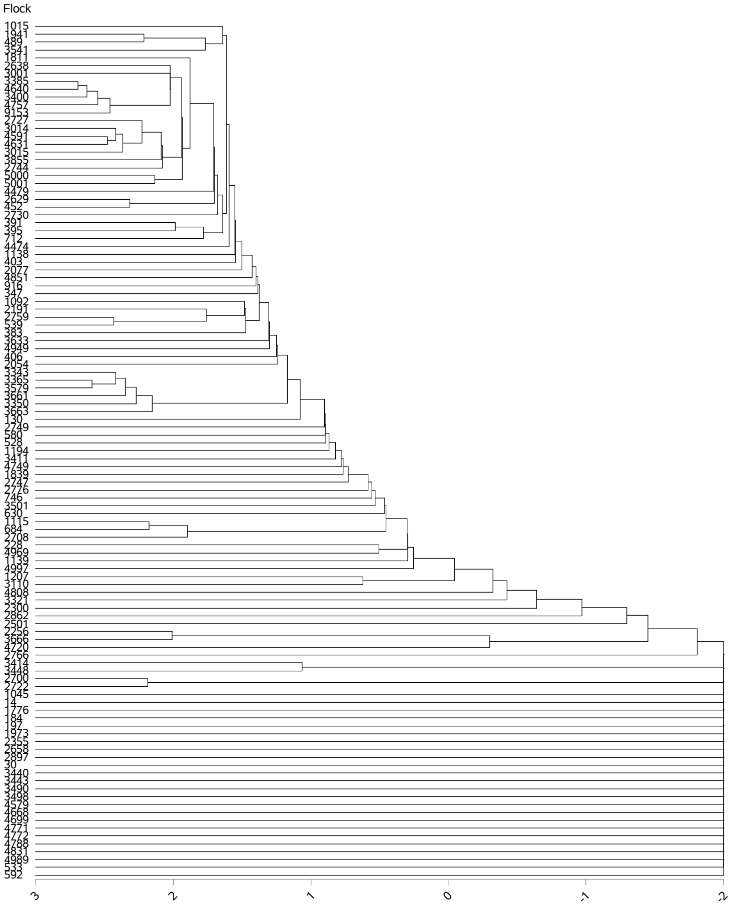
Connectedness for BCS from 2014 to 2020 - GEJob 37284
